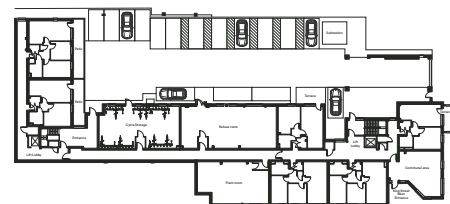
Lower Ground
